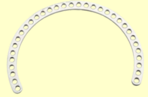
VMS:-611 5/8 Ring Ilizarov External Fixators Size-160mm/180mm
